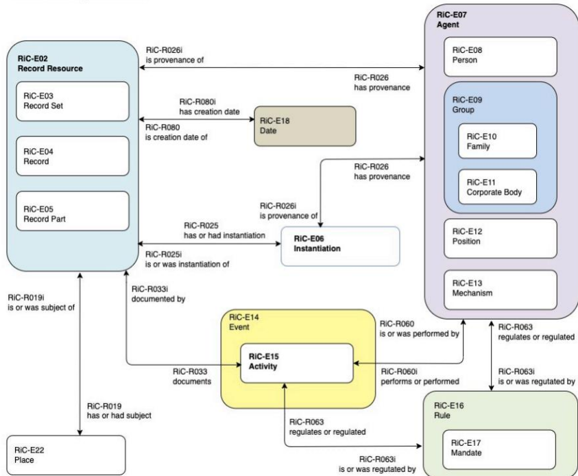
RIC-CM v1.0: a global overview
